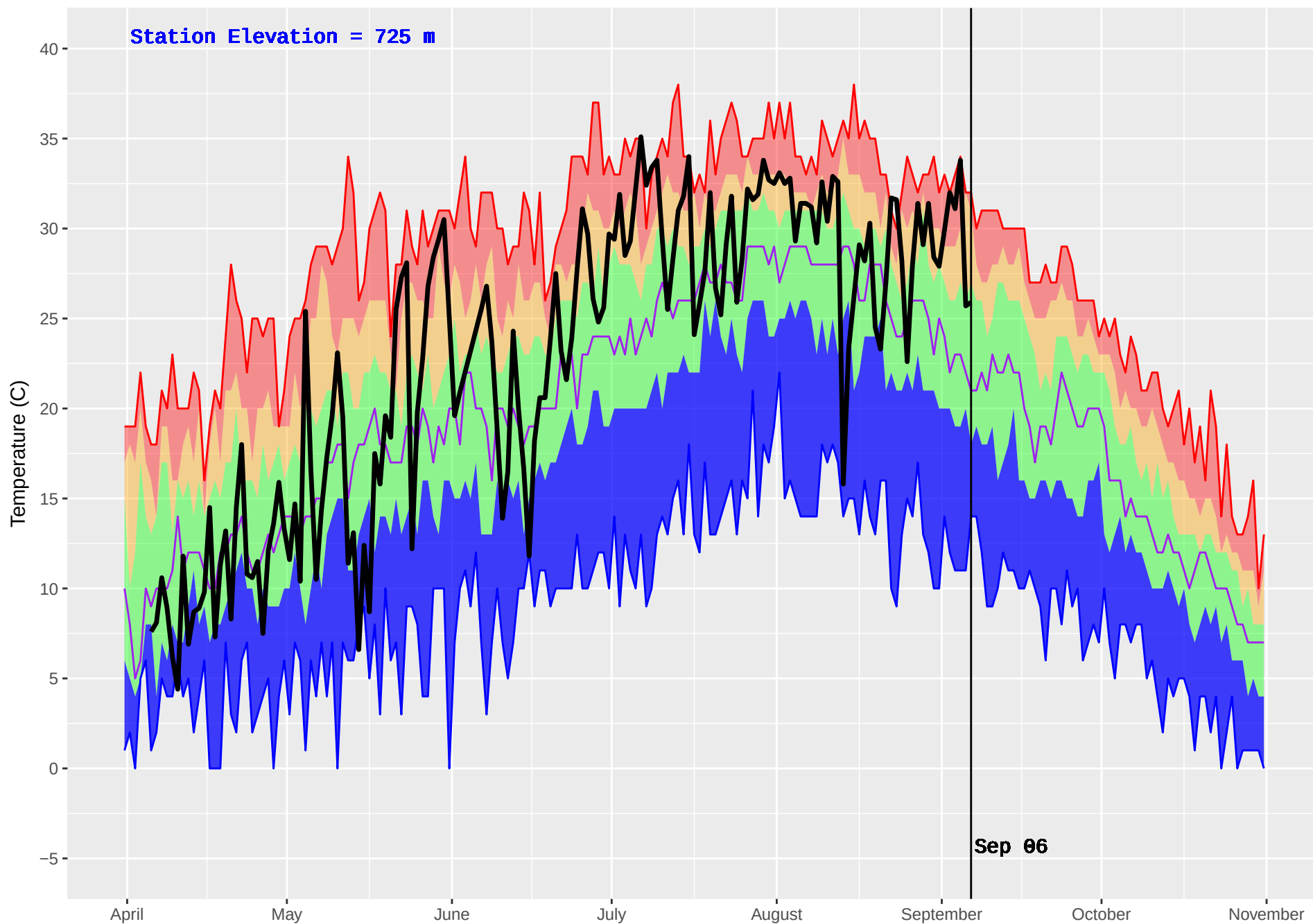
PENDOREILLE (402) : Historical (1986–2016) and Current (2017) Noon Temperature
