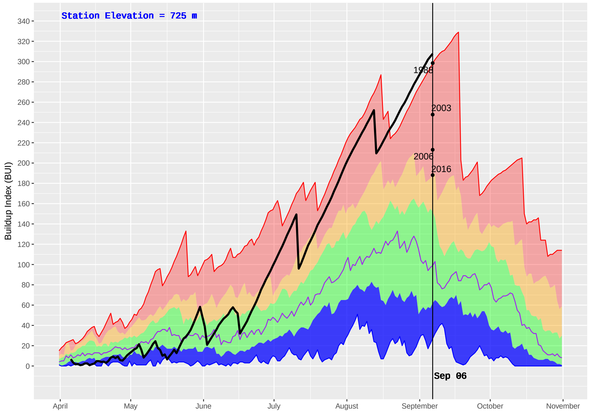
PENDOREILLE (402) : Historical (1986–2016) and Current (2017) Noon Buildup Index (BUI)
